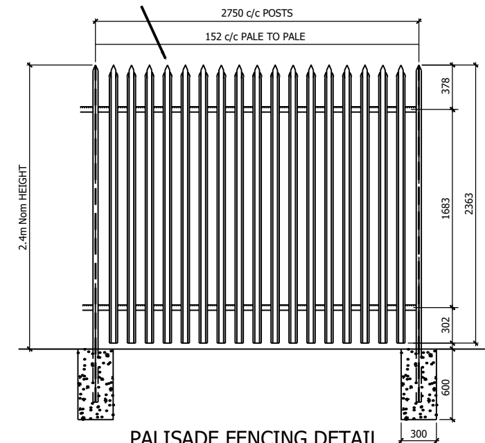
PALISADE FENCING DETAIL
